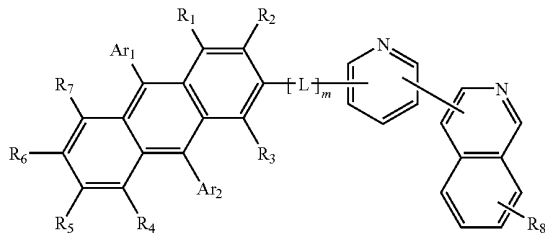
Formula 4
