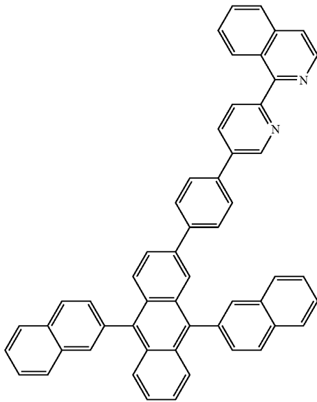
Formula 26
