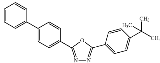
oxadiazole-containing compound
