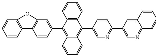
Formula 74
