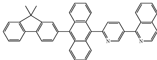
Formula 74
