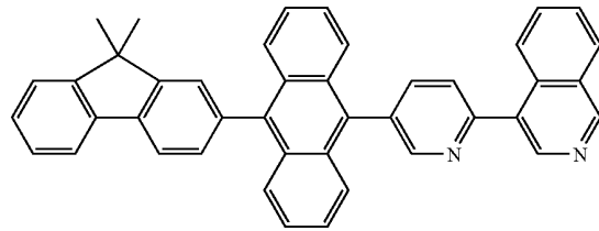
Formula 73
